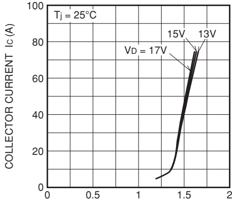
COLLECTOR-CURRENT I_c (A)
