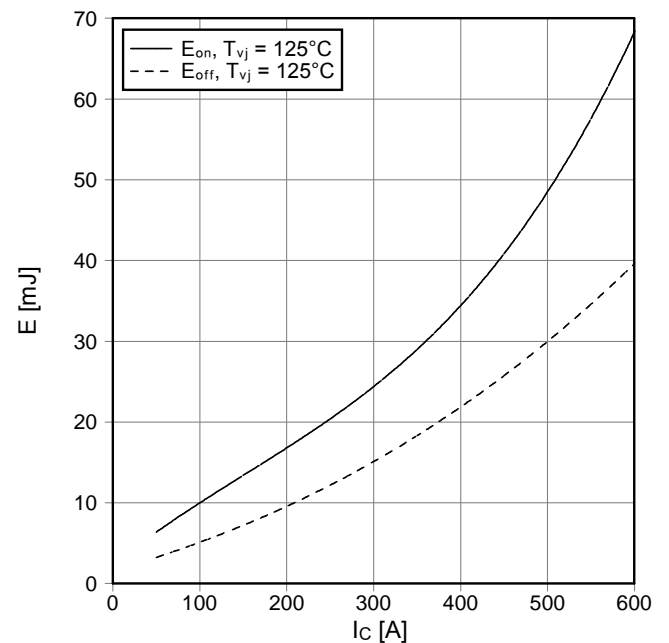
Schaltverluste IGBT-Brems-Chopper switching losses IGBT-brake-chopper E_{on} = f(I_C), E_{off} = f(I_C) V_{GE} = \pm 15\text{ V}, R_{Gon} = 3\ \Omega, R_{Goff} = 3\ \Omega, V_{CE} = 600\text{ V}
