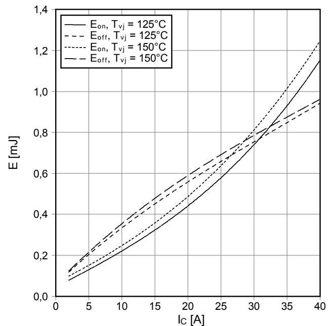
Schaltverluste IGBT-Wechselr. (typisch) switching losses IGBT-inverter (typical) E_{on} = f(I_c) , E_{off} = f(I_c) V_{GE} = \pm 15\text{ V} , R_{Gon} = 18\ \Omega , R_{Goff} = 18\ \Omega , V_{CE} = 300\text{ V}
