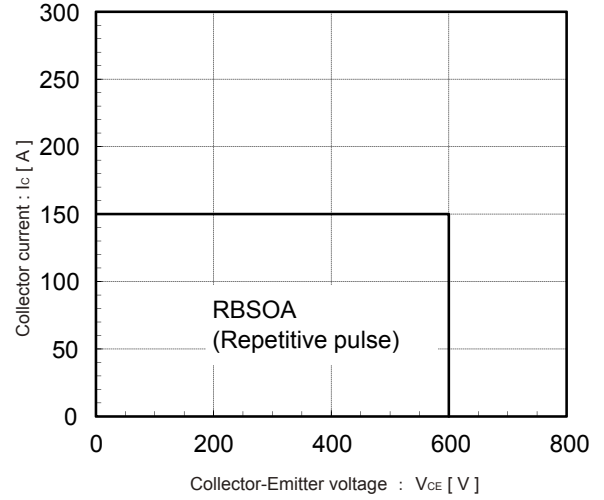
Reversed biased safe operating area V_{CE}=15V, T_j \le 125^\circ C [Main Terminal] (min.)
