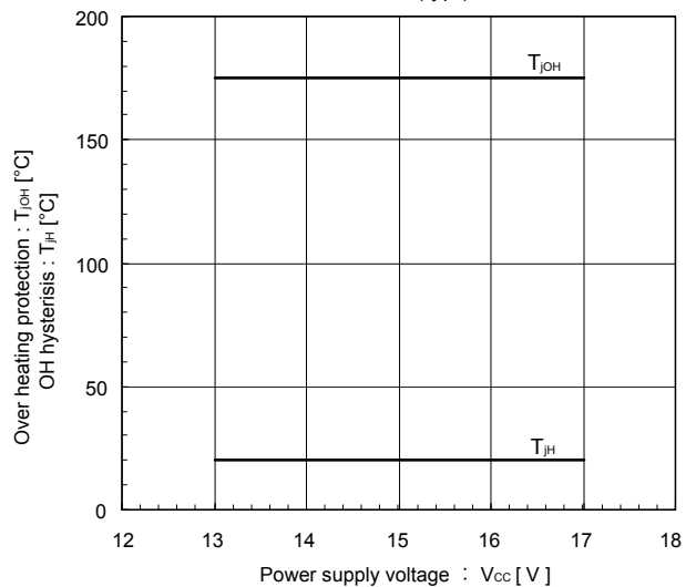
Over heating characteristics T_{\text{JOH}}, T_{\text{JH}} vs. V_{\text{CC}} (typ.)
