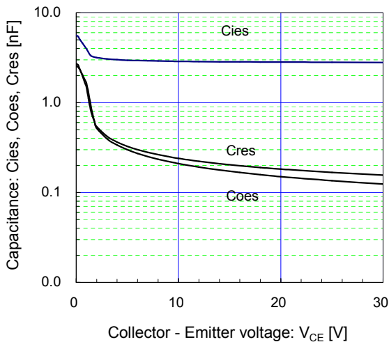
[ Brake ] Capacitance vs. Collector-Emmitter voltage (typ.) VGE=0V, f= 1MHz, Tj= 25 °C
