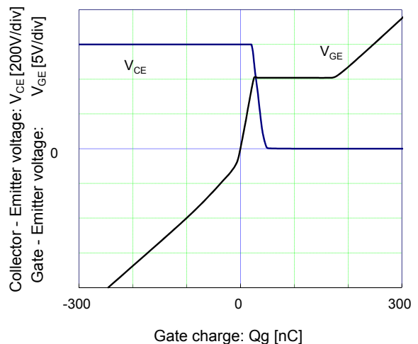
[ Brake ] Dynamic gate charge (typ.) VCC=600V, Ic=35A, Tj= 25 °C
