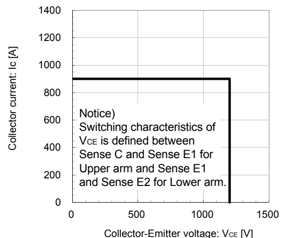
Reverse bias safe operating area (max.) +V_{ge}=15V, -V_{ge}=15V, R_g=0.52\Omega, T_j=150^\circ C
